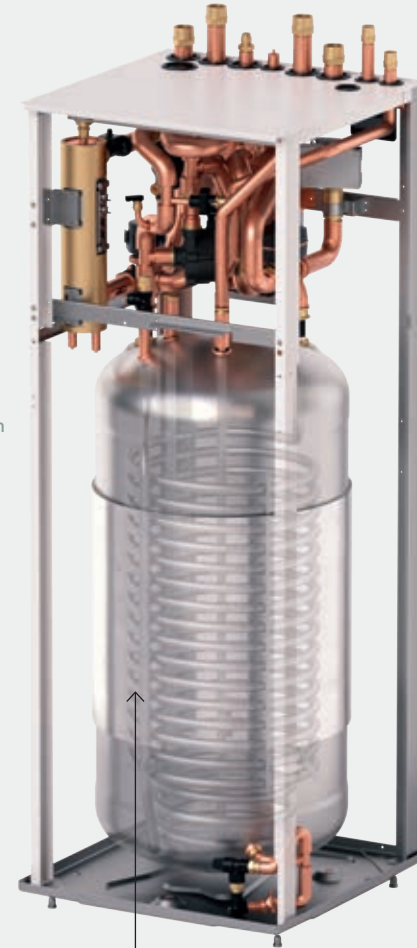
Slimmer, yet same tank capacity. Piping layout at the top in order to maintain large 185 L tank capacity.
